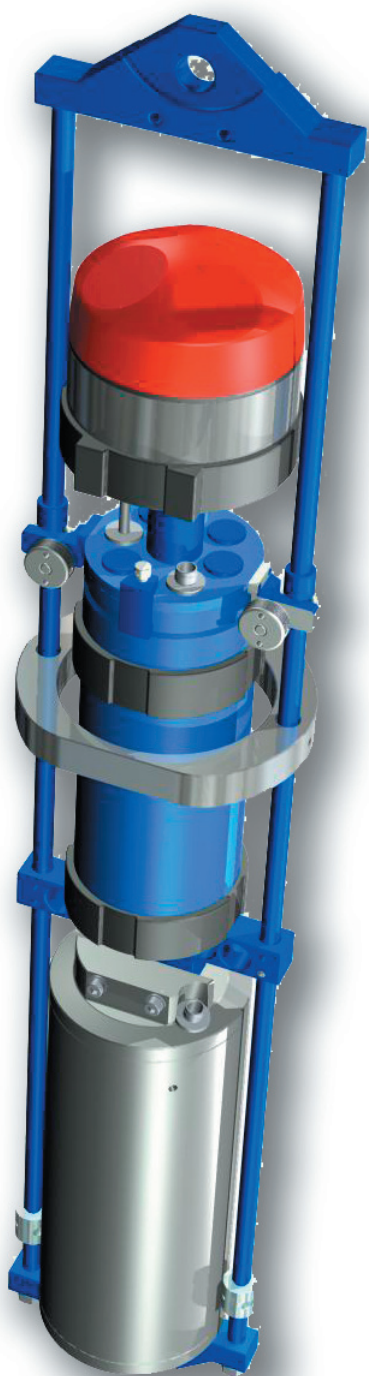
Above: Short battery case mounted in an extended RDCP600 frame
